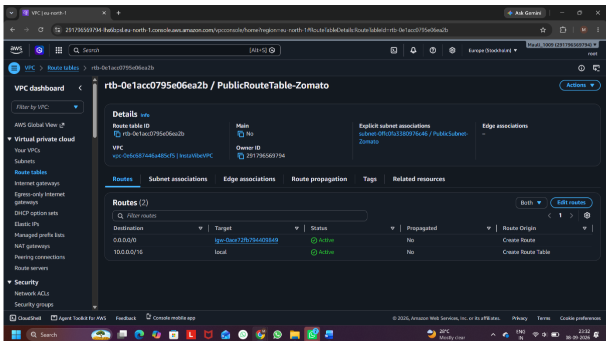
Figure 1: Public Route Table with Internet Gateway Route
