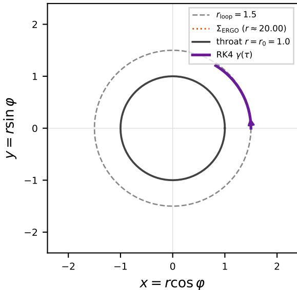
RK4 geodesic ( \Delta\tau = 0.01 , 200 steps)
