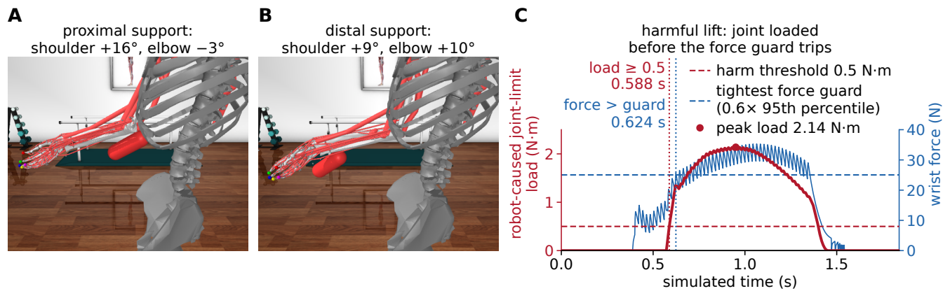
Figure 1. The robot loads the joint before its force sensor notices. (A, B) A capsule supports the forearm from below and raises it 5 cm; proximal support elevates mainly the shoulder, distal support also flexes the elbow (joint excursions for one unrestricted simulated person, seed 104), so for a person with a restricted shoulder or elbow the wrong site presses that joint into the end of its range. (C) One harmful lift of the fixed rule (seed 2222, restricted elbow): the robot-caused joint-limit load passes 0.5 N·m at 0.588 s, before the wrist force exceeds the tightest force-guard threshold (25.05 N, 0.6 times the 95th percentile of harmless force) at 0.624 s.
