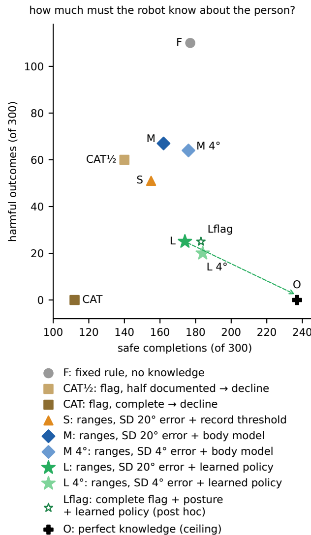
Figure 3. Knowing the person reduces harm, mostly by deciding whom not to lift. Harmful outcomes and safe completions of 300 new persons (round 24, harmful \geq 0.5 N·m; lower right is better) for controllers at six levels of knowledge: none (fixed rule F), half-documented flag, complete flag, ranges with 20° error (S, M, L), ranges with 4° error (M, L) and perfect knowledge (oracle O). The hollow marker (post hoc) is a policy learned from the complete flag and the settled posture only. The dashed arrow is the remaining gap from the learned policy to perfect knowledge. Counts, including declined persons, are in Supplementary Table S4.
