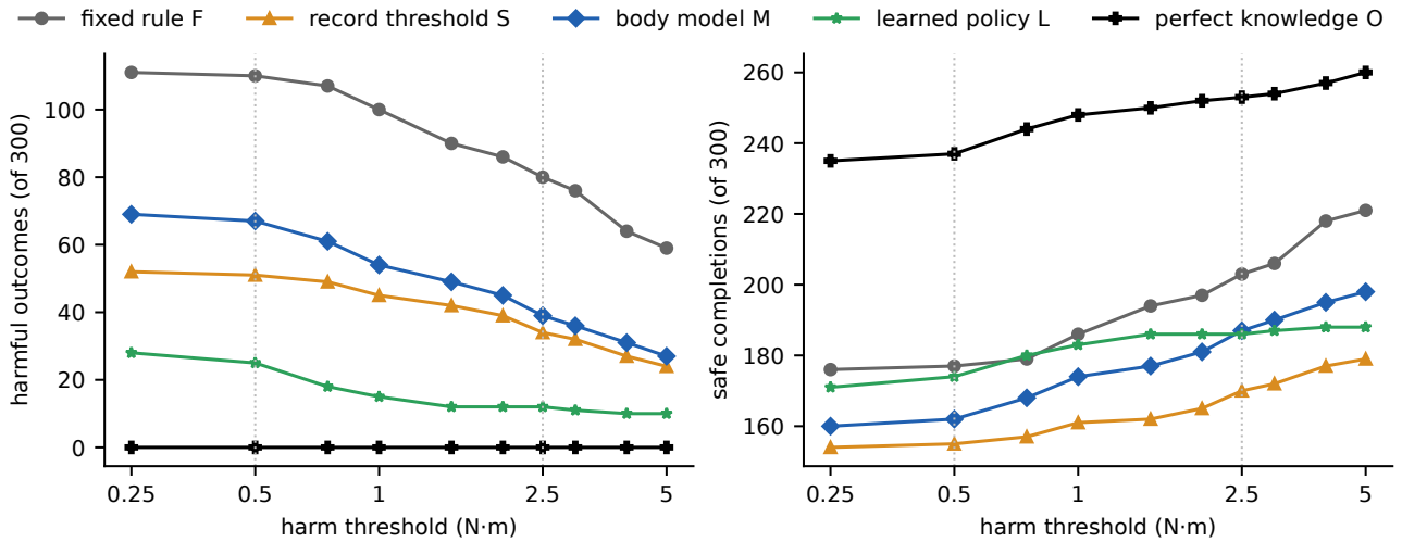
Figure S1. Post hoc sensitivity to the harm threshold (round 24, 300 new persons, record error 20°). Decisions are fixed; only the threshold used to classify outcomes varies. Dotted lines: the prespecified primary (0.5 N·m) and secondary (2.5 N·m) thresholds. Among F, S, M and L, L had the fewest harmful outcomes at every threshold (the complete-flag rule, which declines every flagged person, had none). The price of L's caution grew at lenient thresholds: F completed more lifts safely than L at almost every threshold, and by 8–33 lifts from 1.5 N·m upward (e.g. 203 vs. 186 at 2.5 N·m), while harming many more persons (80 vs. 12).
