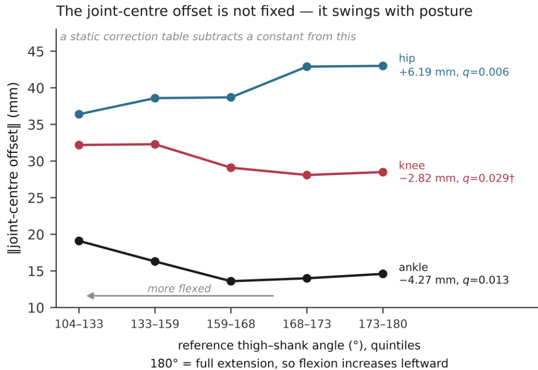
Fig. 2. The joint-centre offset is not fixed but varies with posture. Offset magnitude by quintile of the reference thigh–shank angle ( 180^\circ = full extension for the three-point angle used here). Highest minus lowest quintile: hip +6.19 mm ( q = 0.0065 ), knee -2.82 mm ( q = 0.029^\dagger ), ankle -4.27 mm ( q = 0.013 ), each corrected within the thirteen-test posture family; ^\dagger marks the one that does not survive the arbitrary-dependence sensitivity of Table S5.
