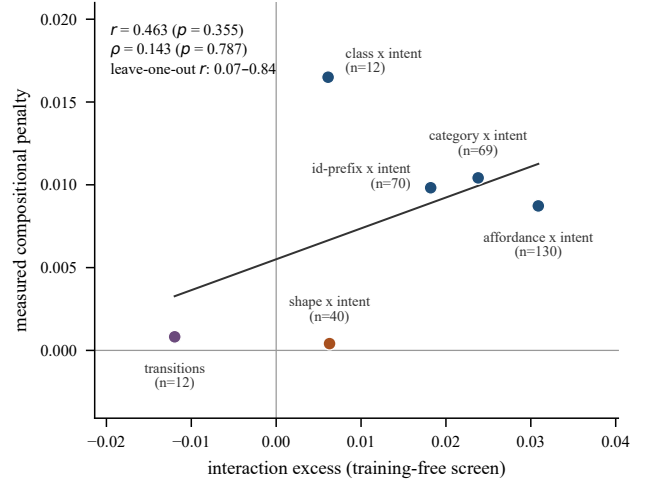
Fig. 1. A statistic computed on raw data factors, without training anything, against the compositional penalty each axis was measured to carry by a full paired sweep. Every axis with a measurable penalty lies right of zero and none lies left of it, so the statistic separates presence from absence; the scatter within the right-hand group is what it does not predict. DexYCB is absent because its sweep could not have measured what it claimed (§V-B).
