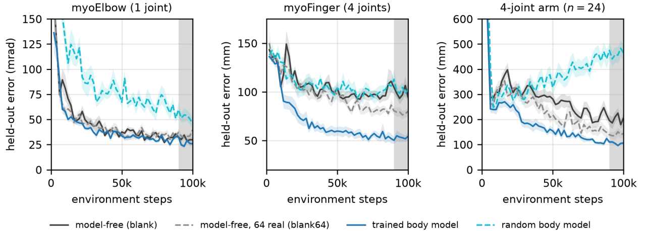
Fig. 4. Learning curves with the trained body model (blue), a random body model in the same machinery (cyan, dashed) and the two model-free baselines (grey). On the four-joint arm the random model ends far above model-free learning while the trained model ends far below it. First evaluation at 2,000 steps. Held-out error, mean, band \pm 1 SE; grey band: the scored window.
