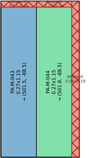
Baldosa M-27 · 2 pza(s)
