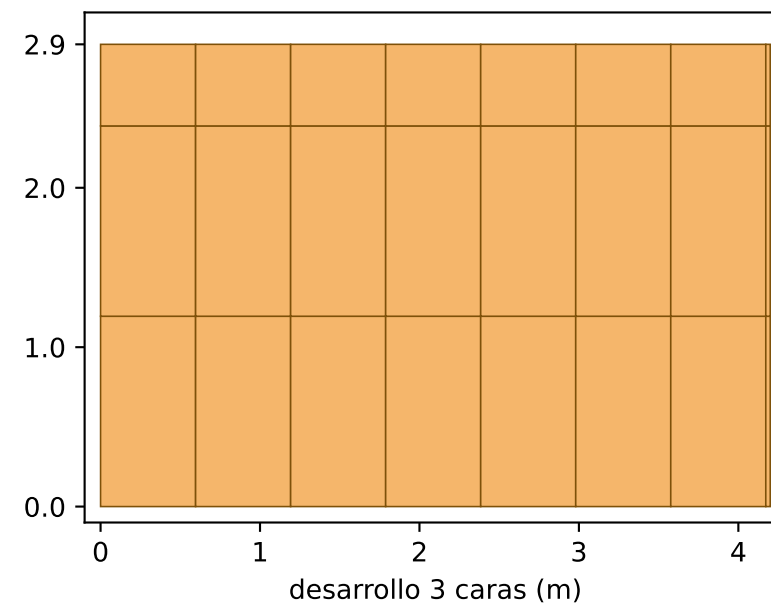
Regadera 3 (P.A.) muro 2.90 m × 4.20 ml = 12.18 m 2
