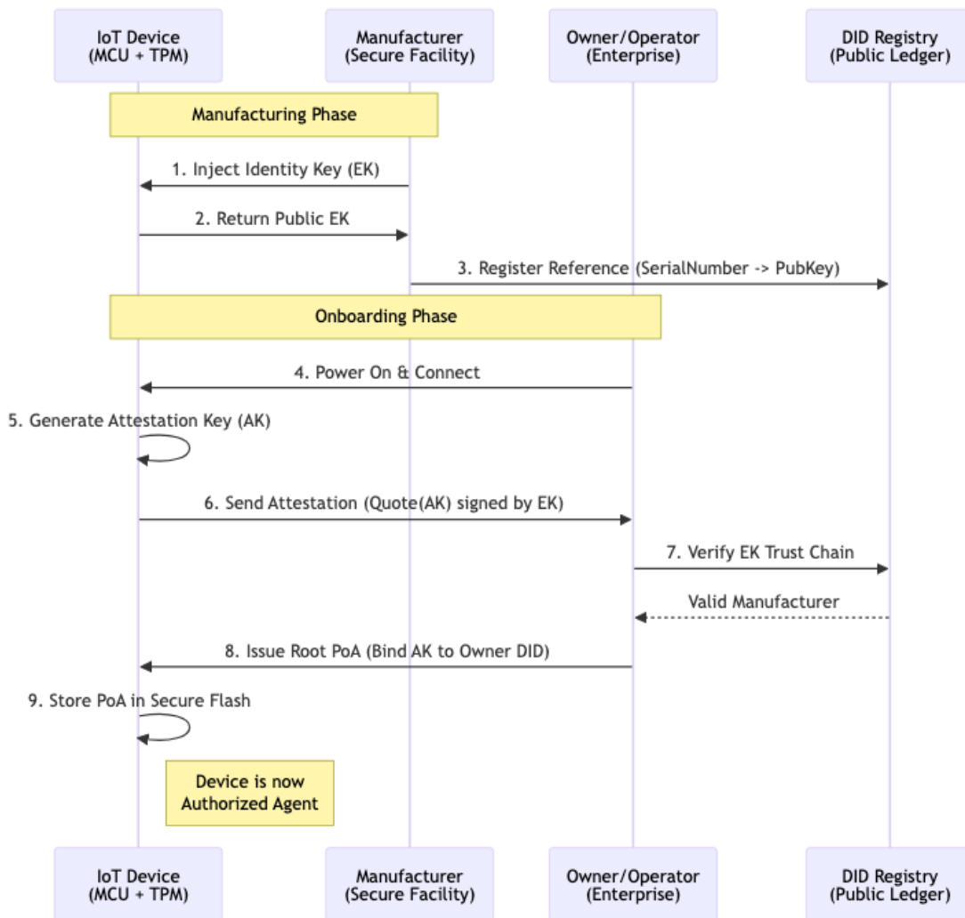
Figure 11.2: Device Trust Bootstrap
