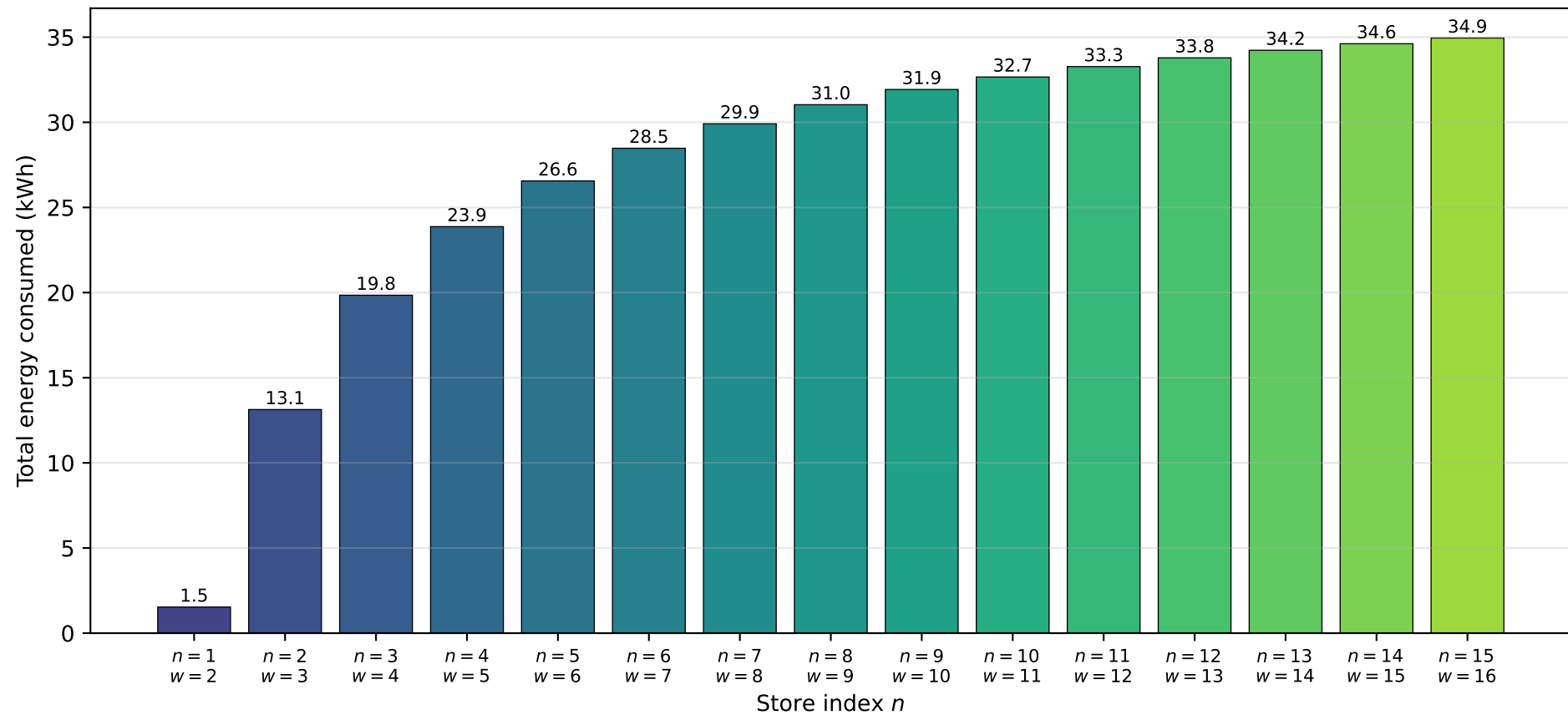
Per-store total energy consumption at final iteration (Adaptive \alpha_0 = 5 )
