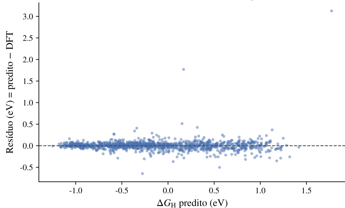
schnet_v2_seed42 - residual vs pred
