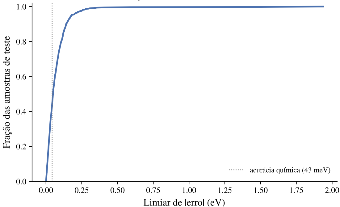
mace_ft_stageA_v2_seed42 - cumulative error
