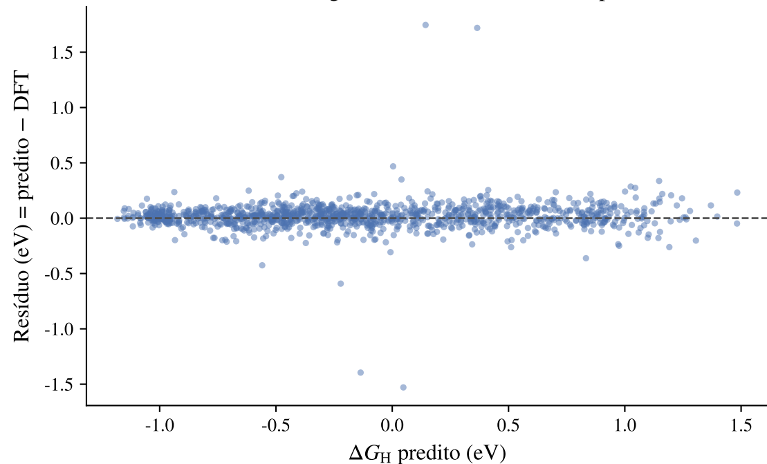
mace_ft_stageA_v2_seed1 - residual vs pred
