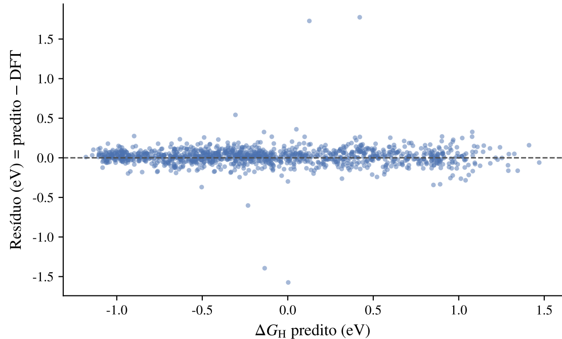
mace_ft_stageA_v2_seed3 - residual vs pred
