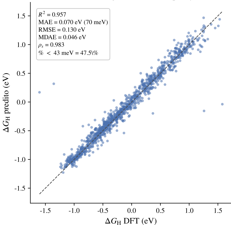
mace_ft_stageA_v2_seed4 - parity
