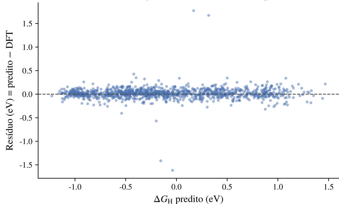
mace_ft_stageA_v2_seed4 - residual vs pred
