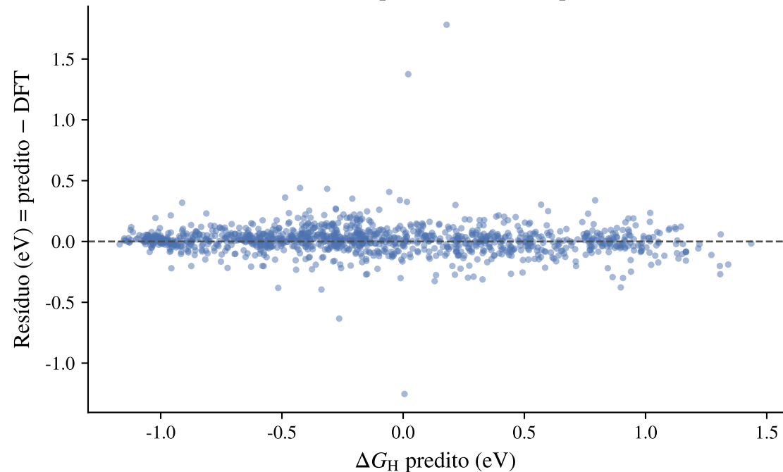
etr_emb_top100 - residual vs pred
