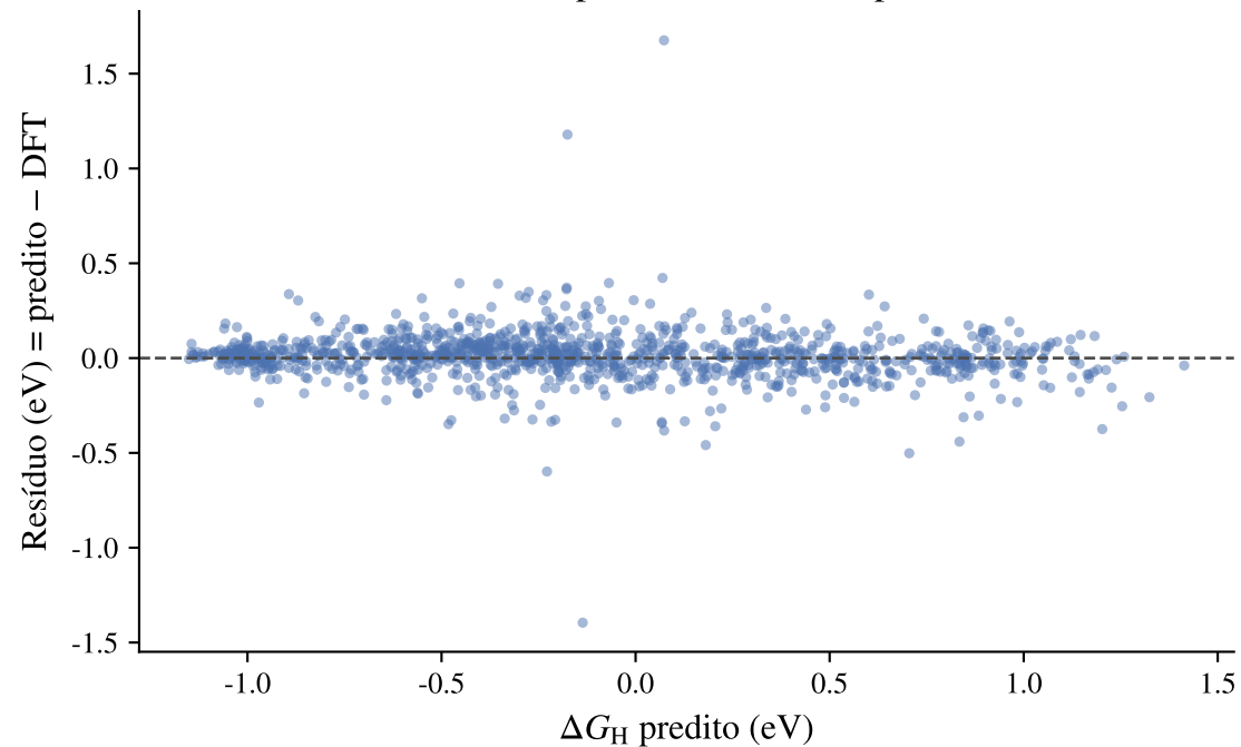
etr_emb_pca95 - residual vs pred
