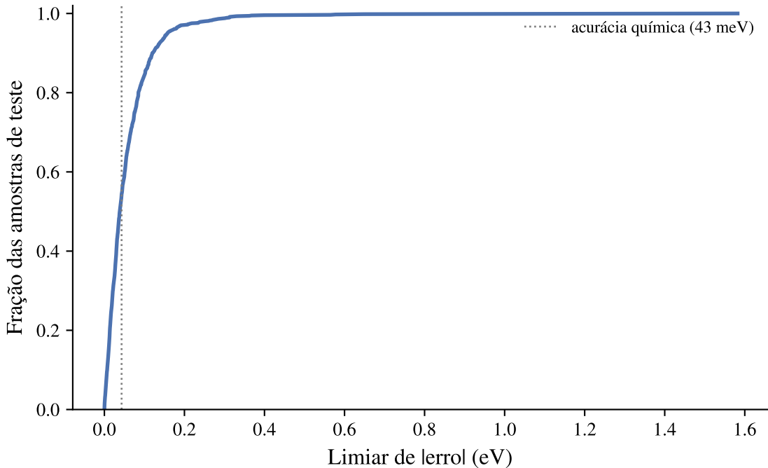
ensemble_eval - cumulative error
