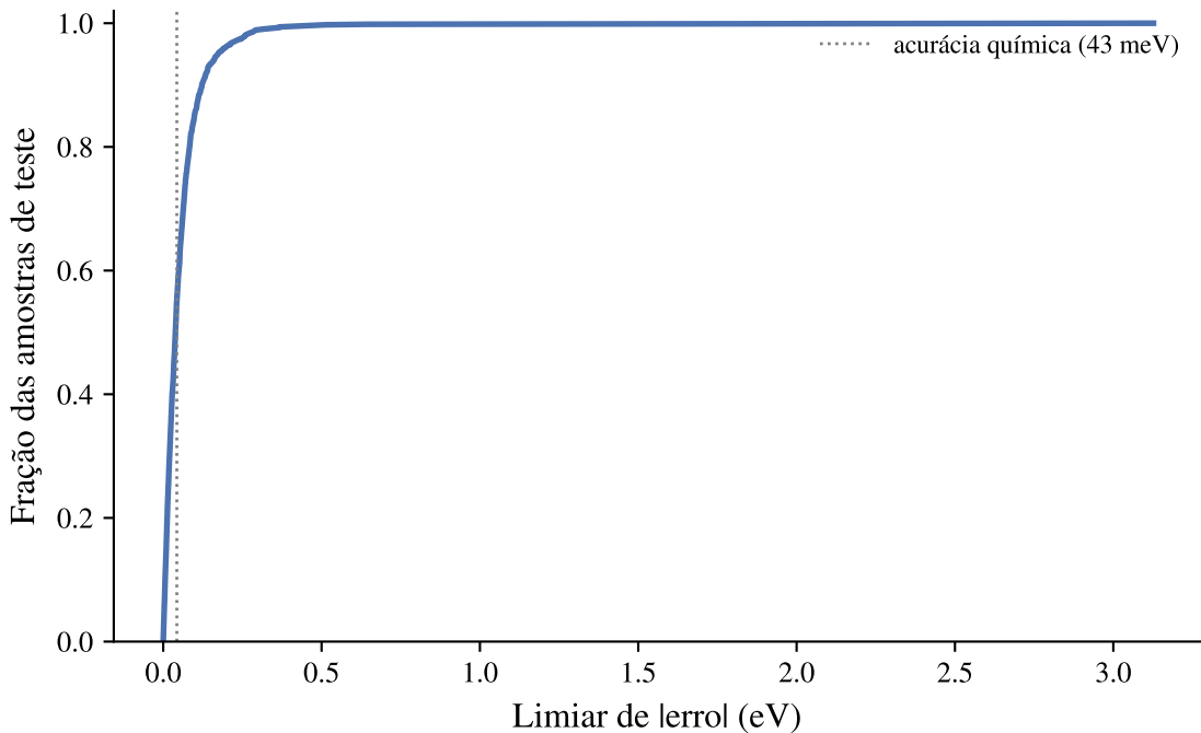
schnet_v2_seed42 - cumulative error
