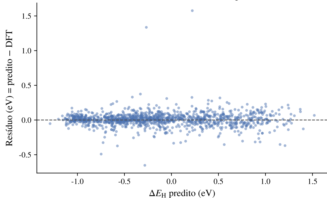
schnet_v2_seed1 - residual vs pred
