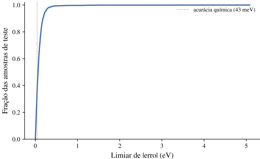
schnet_v2_seed2 - cumulative error
