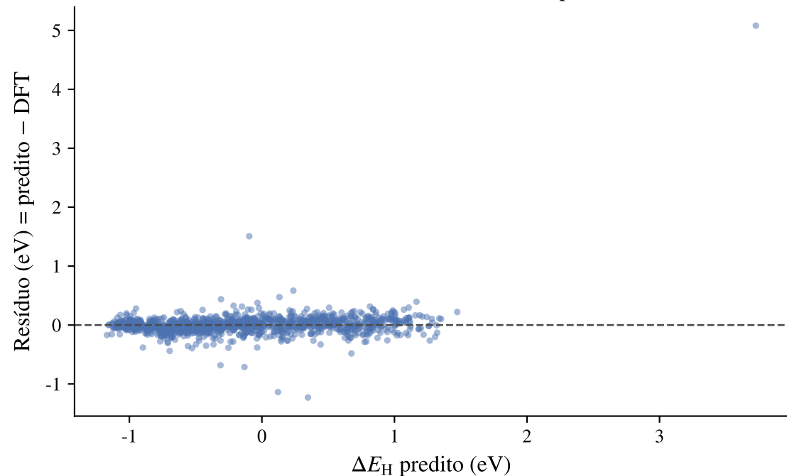
schnet_v2_seed2 - residual vs pred
