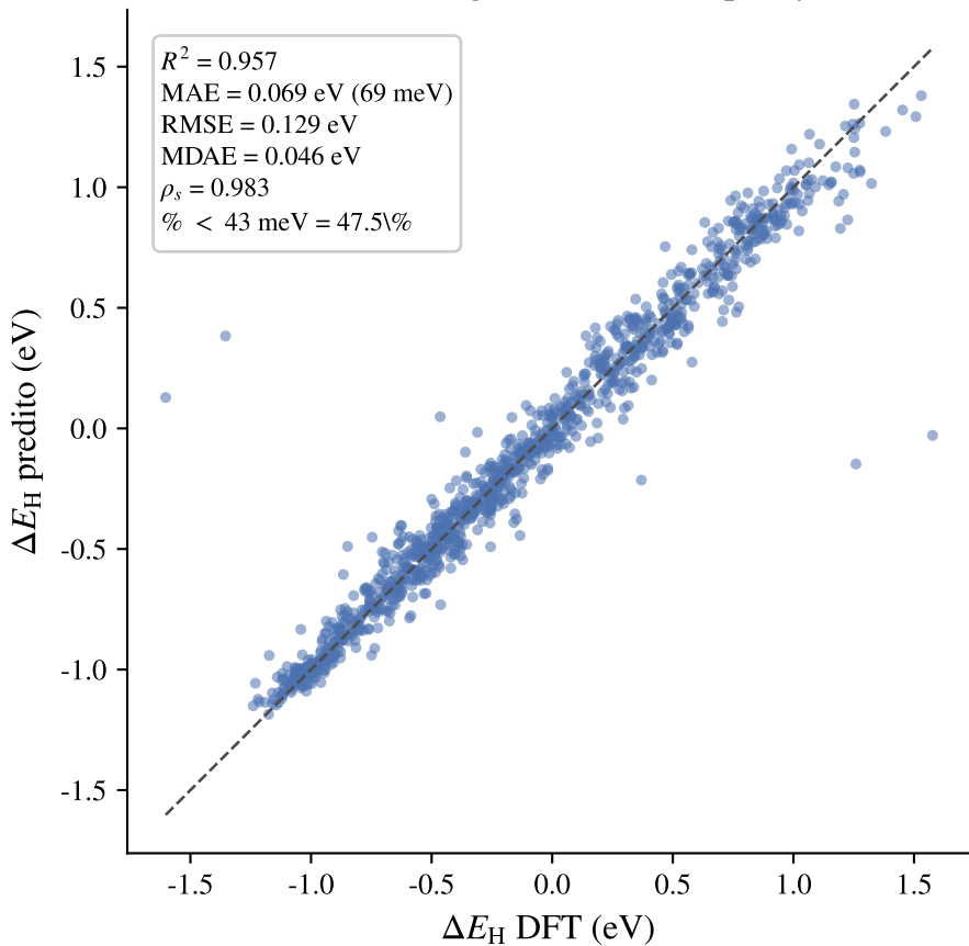
mace_ft_stageA_v2_seed2 - parity
