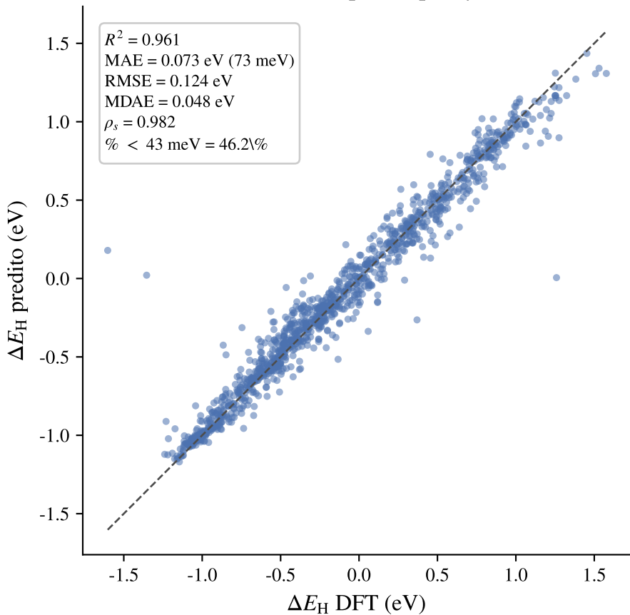
etr_emb_top100 - parity
