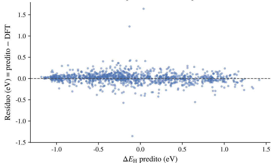
etr_emb_pca90 - residual vs pred
