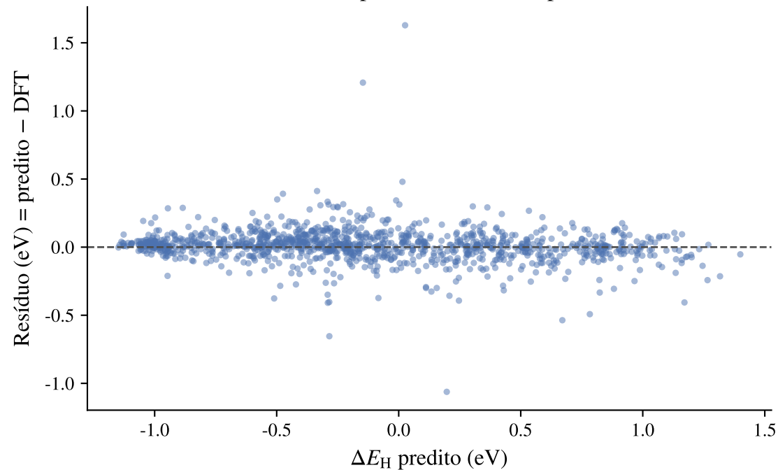
etr_emb_pca99 - residual vs pred
