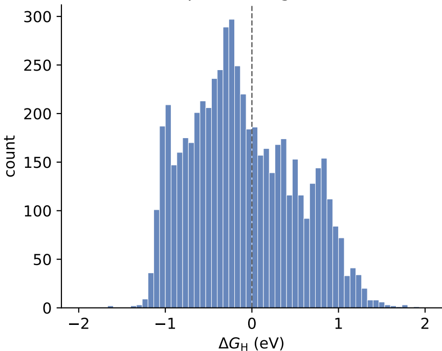
HER adsorption energies (n=5860)
