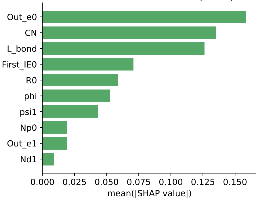
Feature importance (mean |SHAP|)
