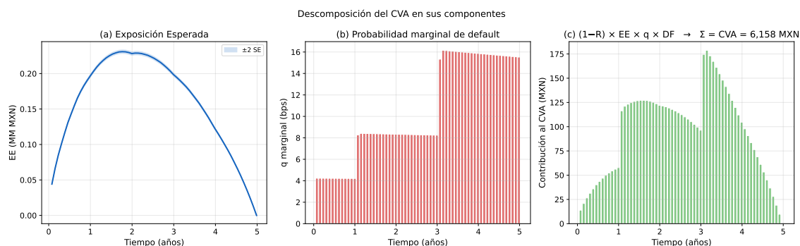
Figure 7: The reference swap: expected exposure, marginal default probability and each period's discounted contribution; the bars add up to the 6,158 MXN CVA. Axis labels in Spanish.
