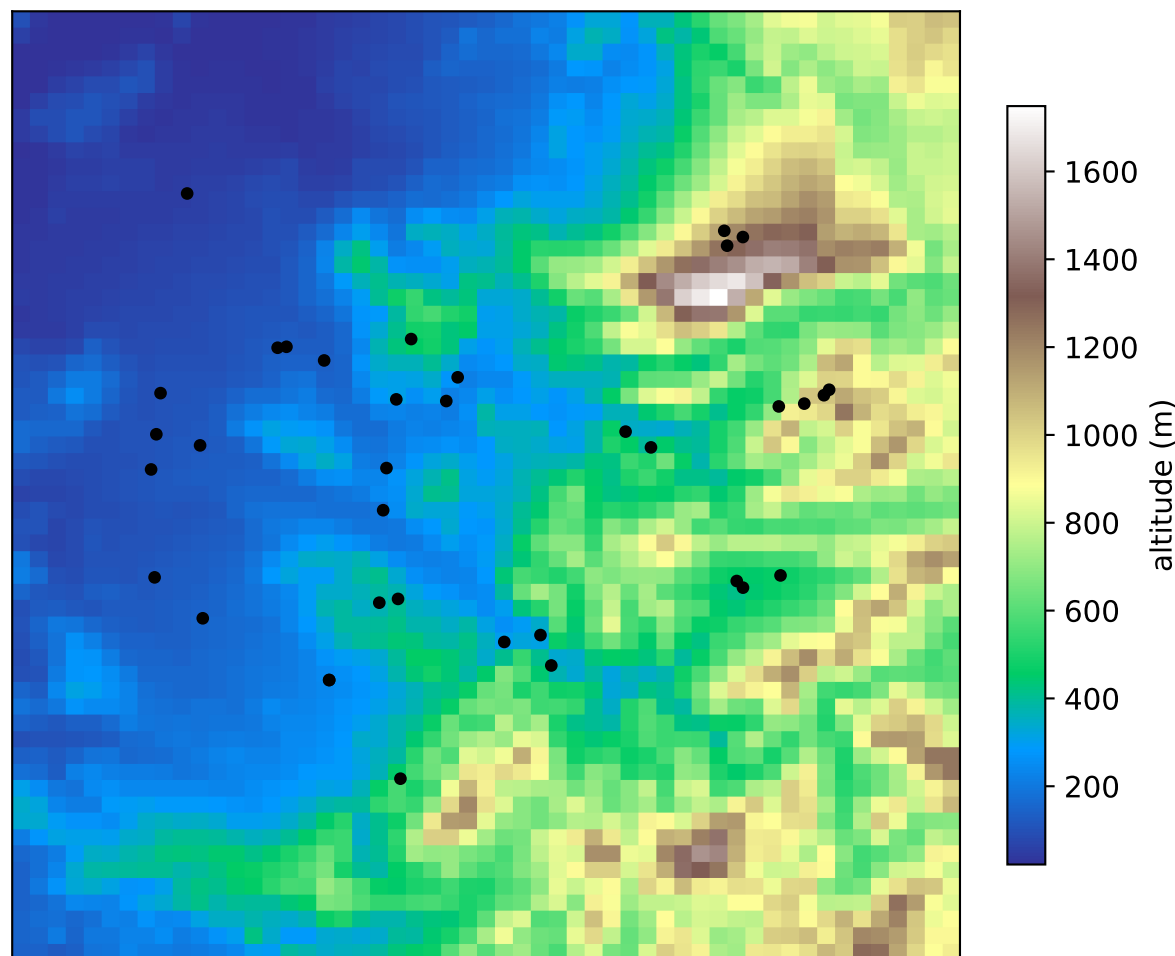
③ CERRA 5,5 km (background)
