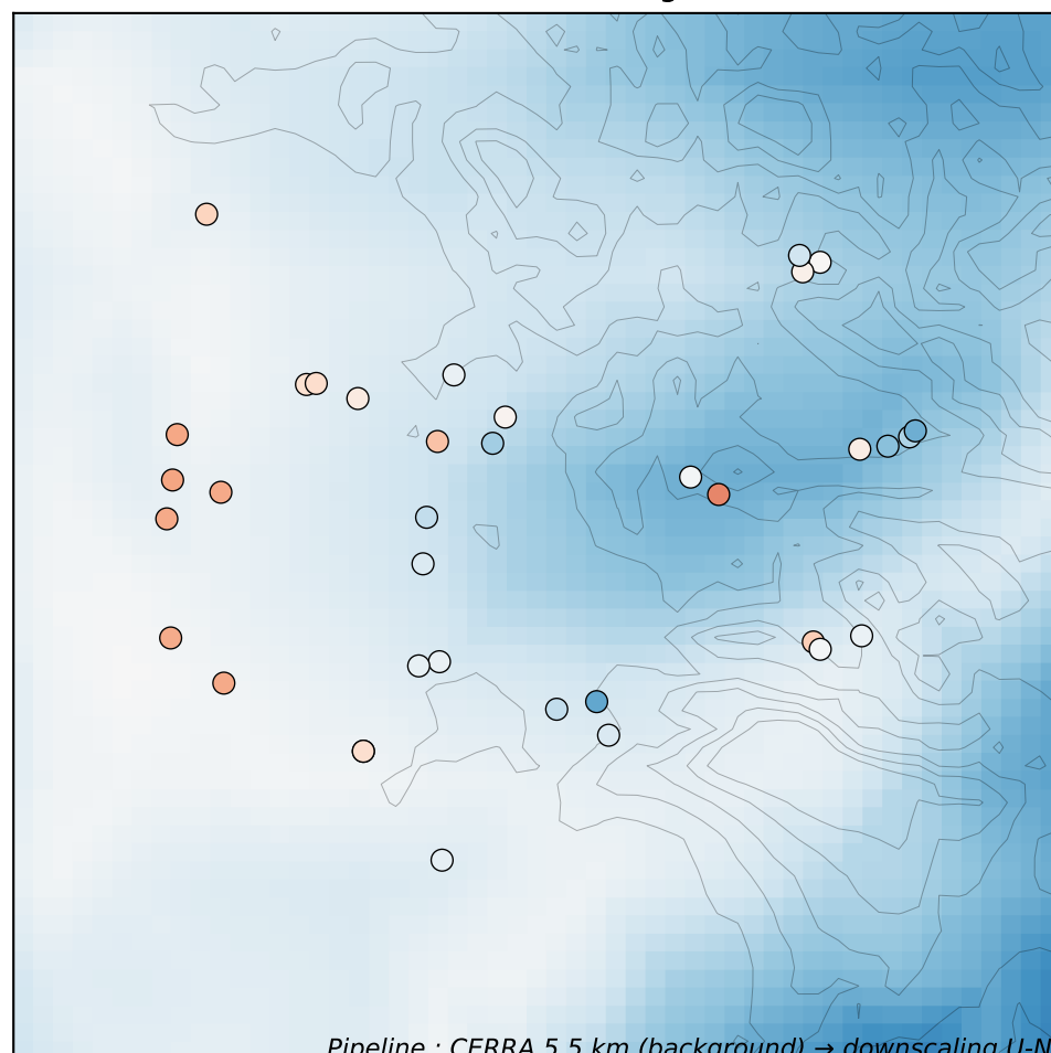
③ CERRA 5,5 km (background)
