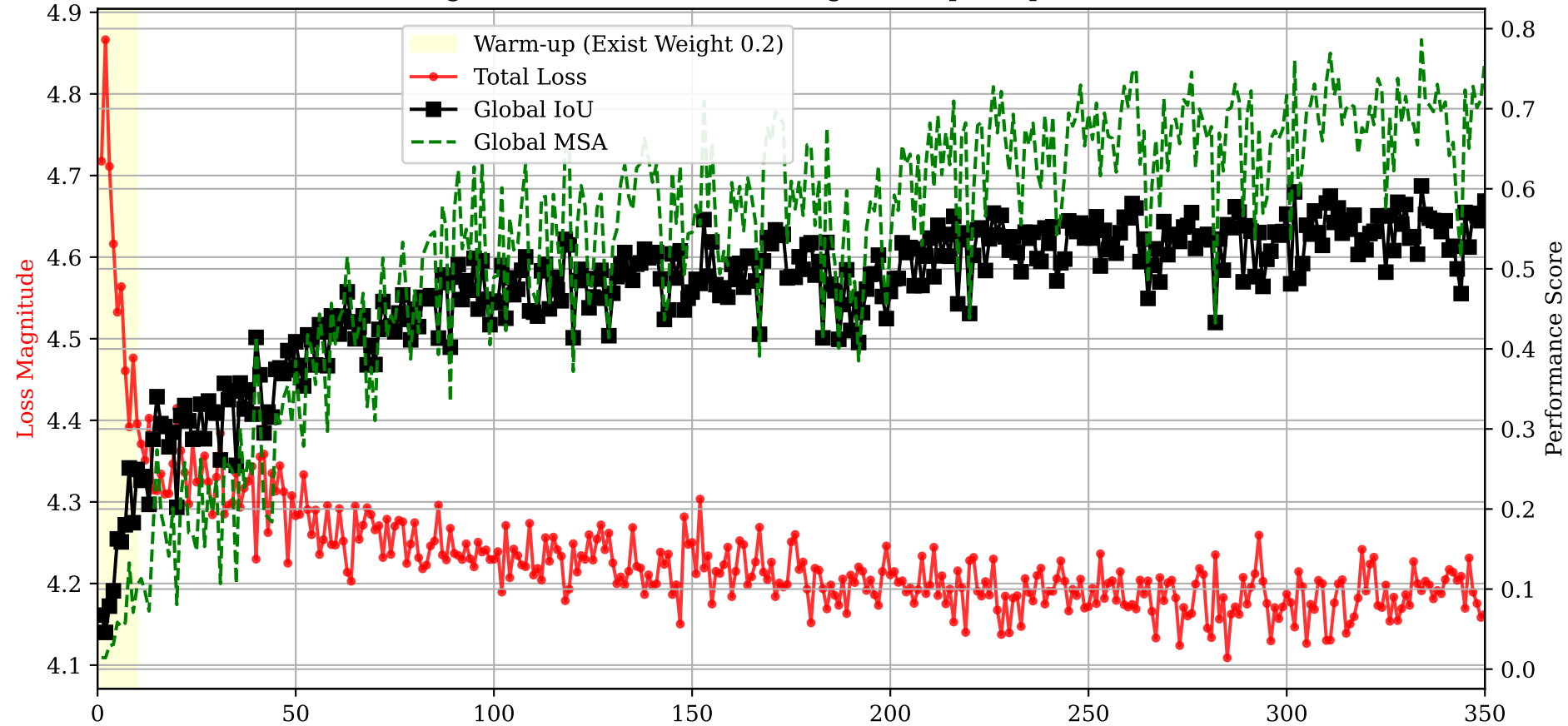
Figure 1: Global Error Convergence (Up to Epoch 350)
