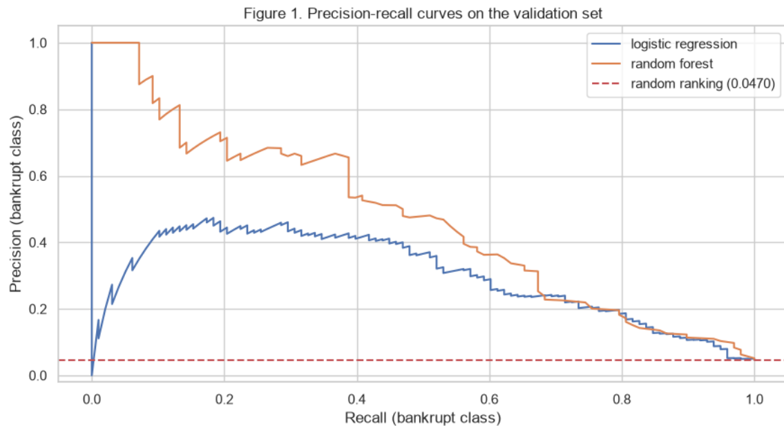
Precision-Recall Curves of the Two Learned Models on the Validation Set
