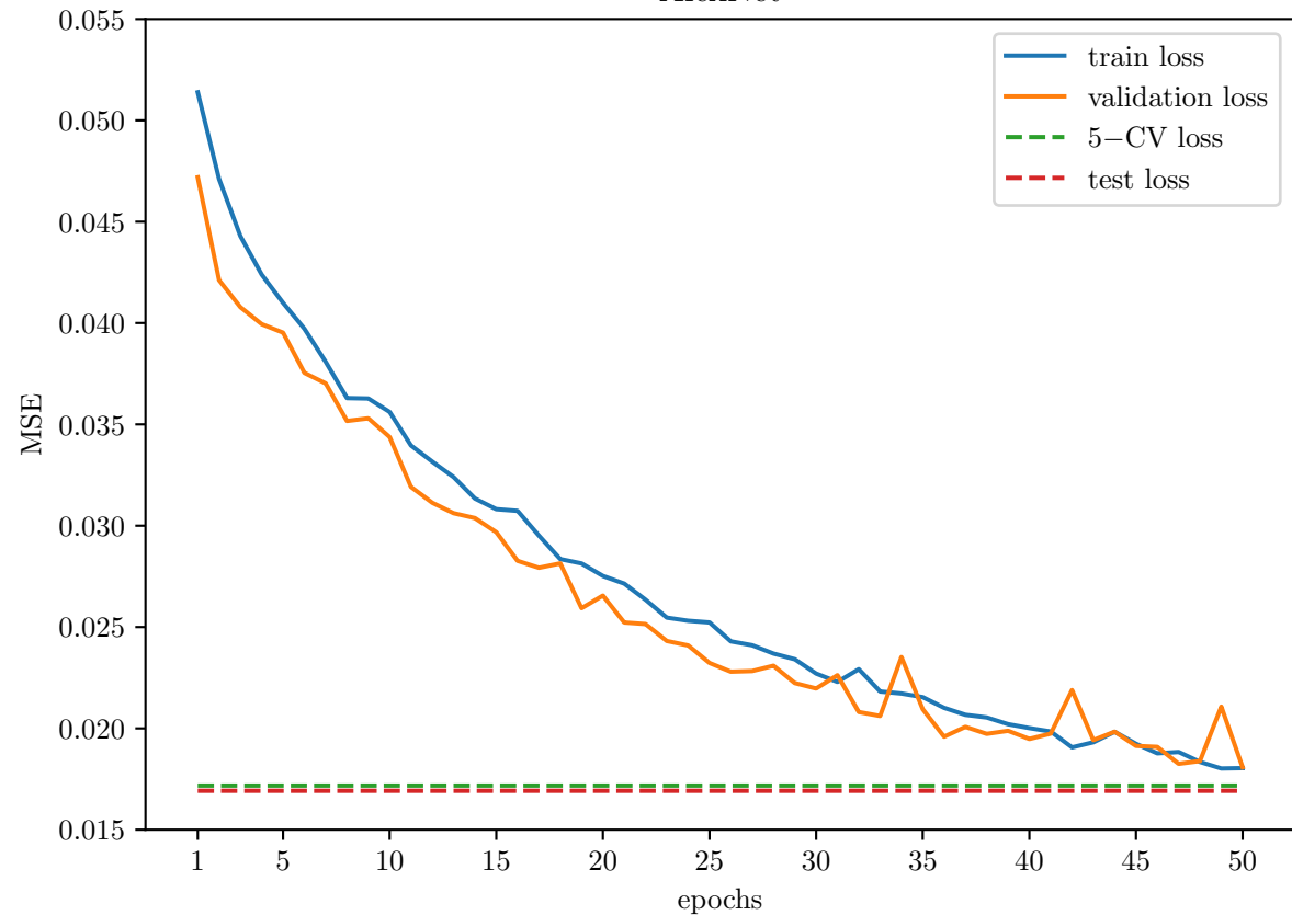
AlexNet
