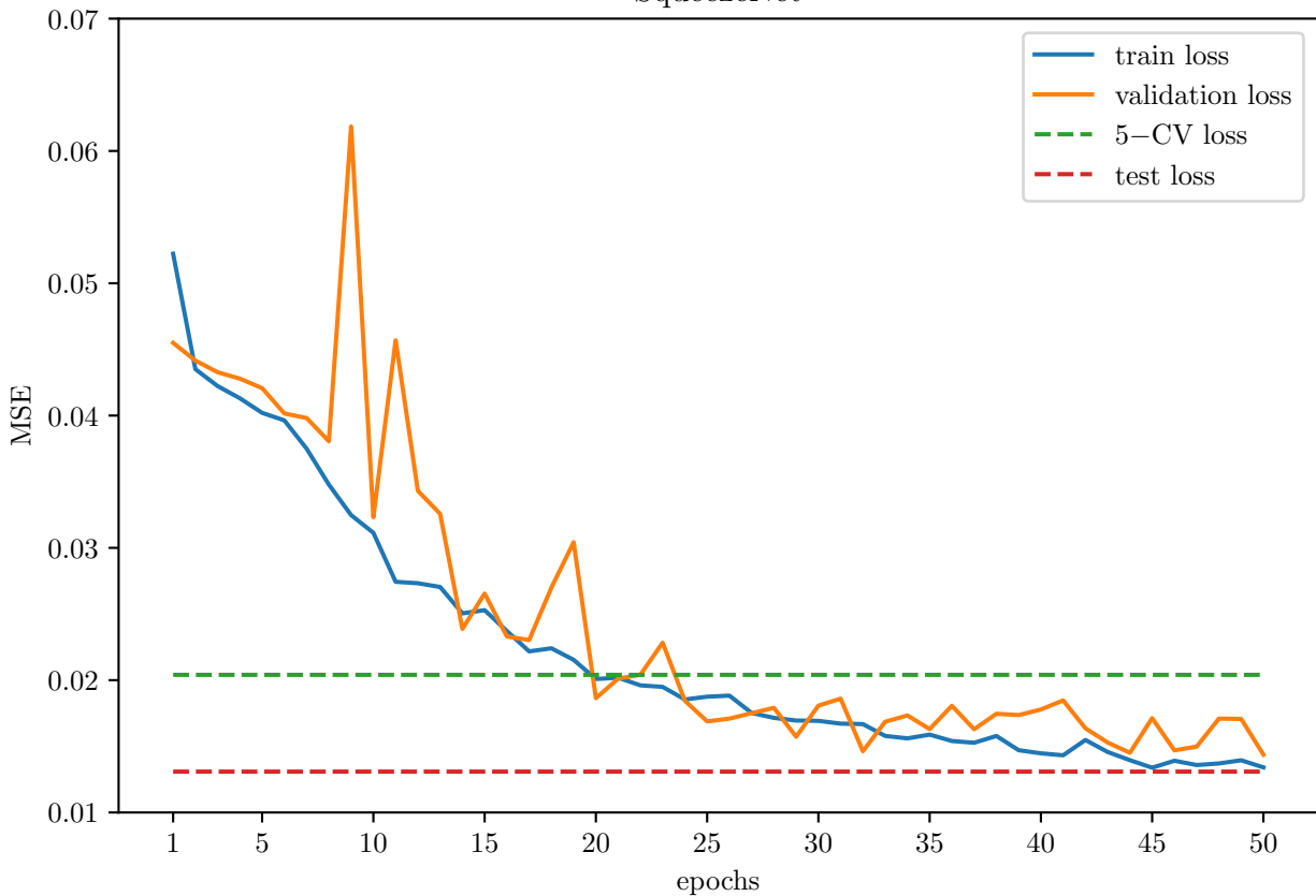
SqueezeNet
