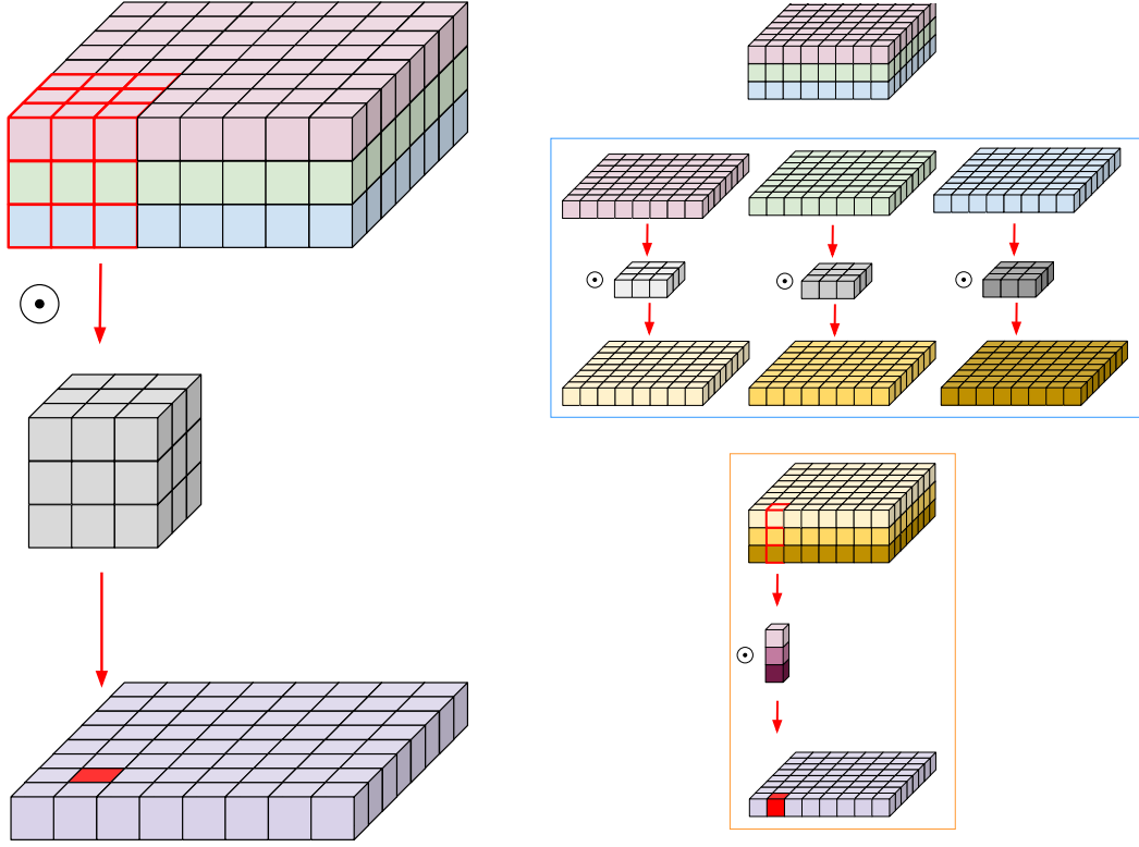
Figure 8: Standard Convolution (left) and Depthwise+Pointwise Convolution (right). The Depthwise conv. is highlighted in light blue while Pointwise conv. in orange [9].
