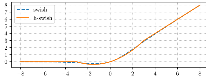
Figure 9: Swish and h-swish
