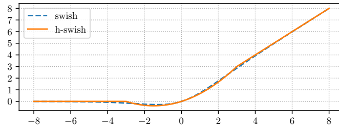
Figure 9: Swish and h-swish
