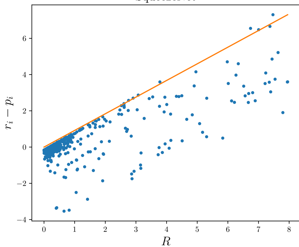
SqueezeNet
