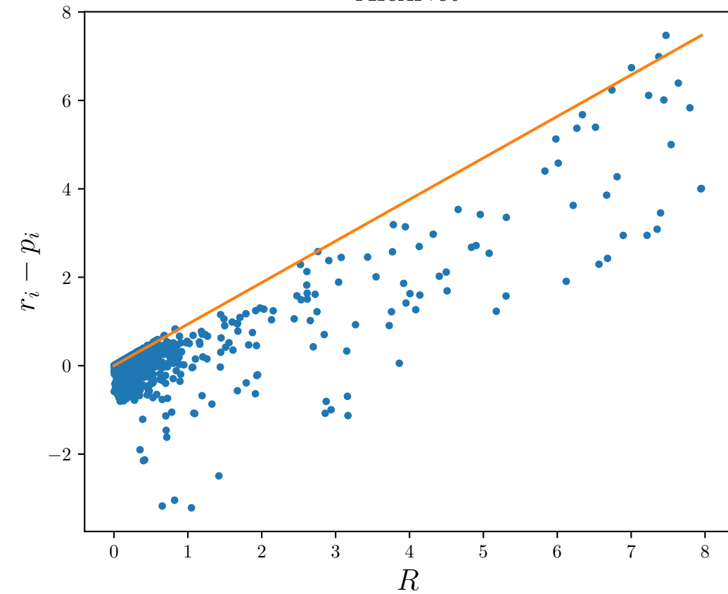
AlexNet
