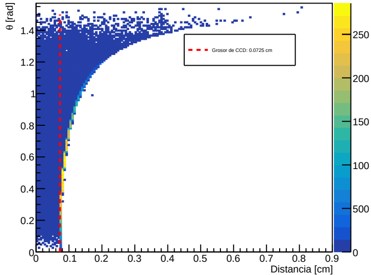
Lvs \theta (Geant4)
