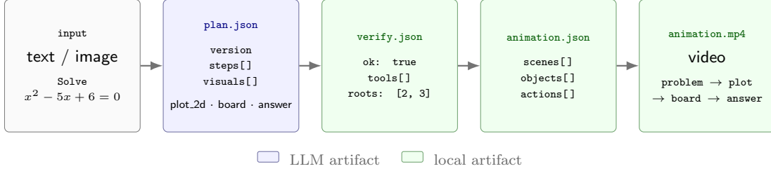
Figure 2: Quadratic run as pictographs. Boxes sketch the JSON shape (keys / tool names), not complete file contents.
