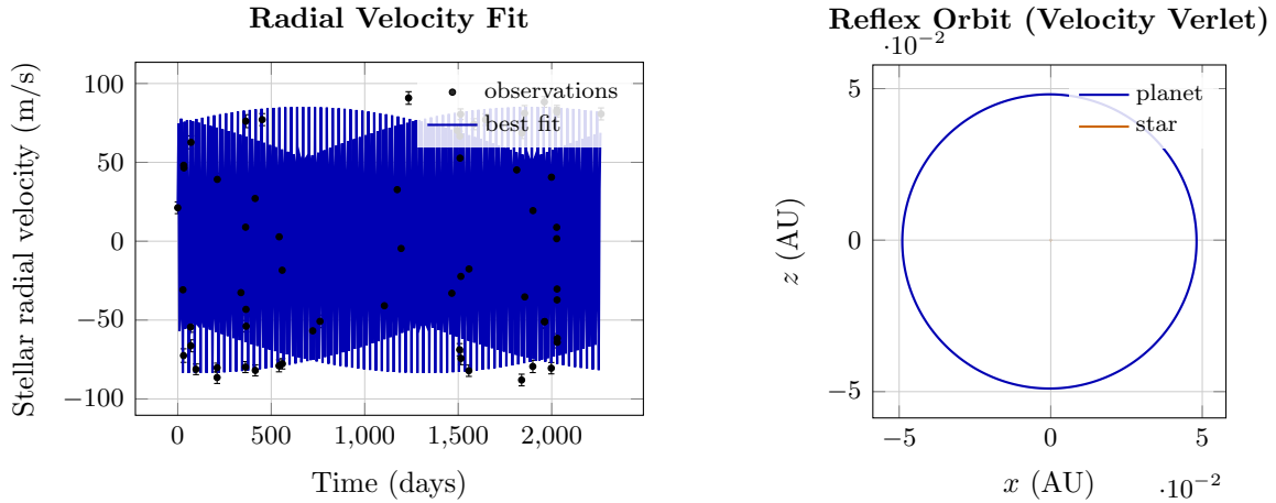
Figure 3: Keplerian fit to the public HD 209458 radial-velocity series of Butler et al. [15].
