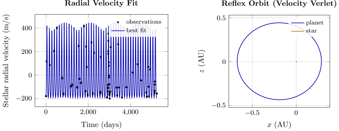
Figure 4: Keplerian fit to the public 70 Vir radial-velocity series of Butler et al. [15].
