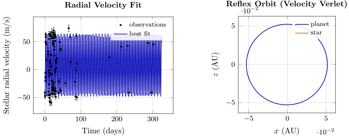
Figure 2: Keplerian fit to the public 51 Peg radial-velocity series of Marcy et al. [14]. Left: radial-velocity time series and best-fit model. Right: corresponding barycentric orbit. Fits for HD 209458, 70 Vir, and HD 3651 are shown in Appendix B.
