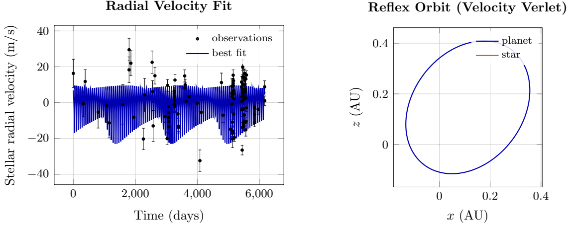
Figure 5: Keplerian fit to the public HD 3651 radial-velocity series of Butler et al. [15].
