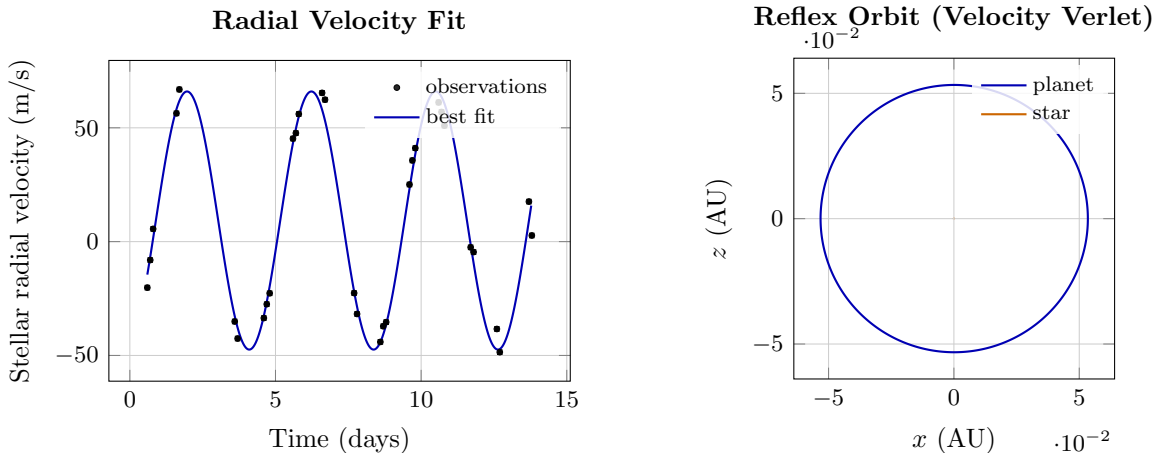
Figure 2: Keplerian fit to the star0 Doppler observations. Left: radial-velocity time series and best-fit model. Right: corresponding barycentric orbit. Fits for star1 – star3 are shown in Appendix A.
