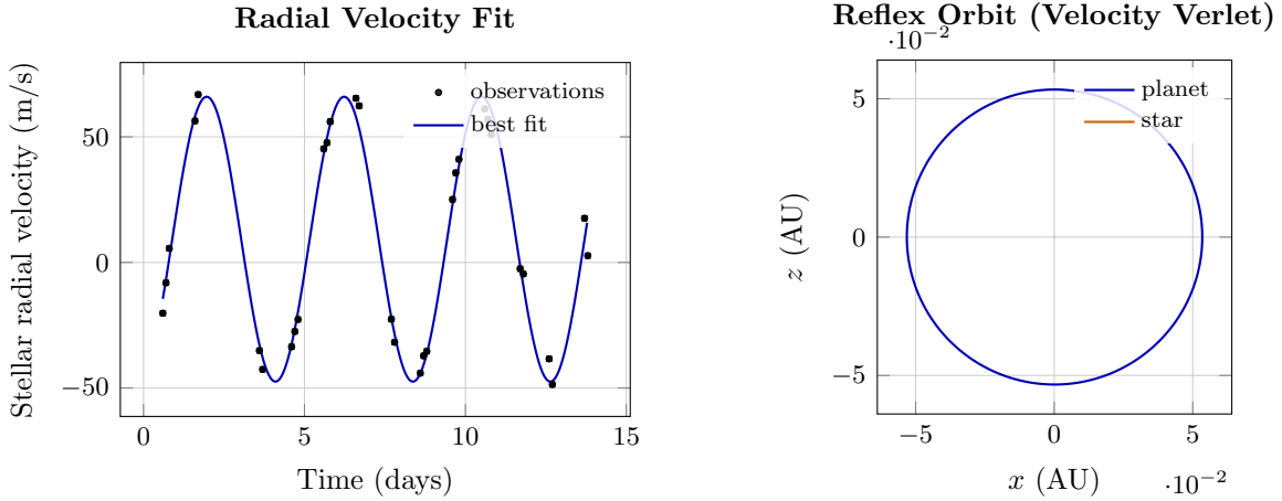
Figure 2: Keplerian fit to the star0 Doppler observations. Left: radial-velocity time series and best-fit model. Right: corresponding barycentric orbit.
