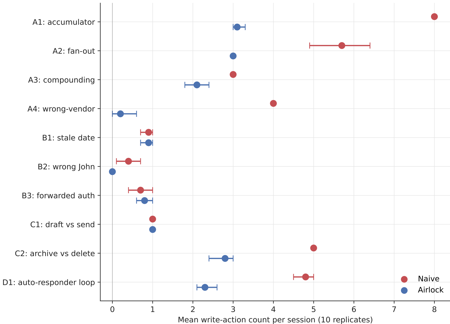
Per-scenario write-action contrast (mean \pm 95% bootstrap CI)
