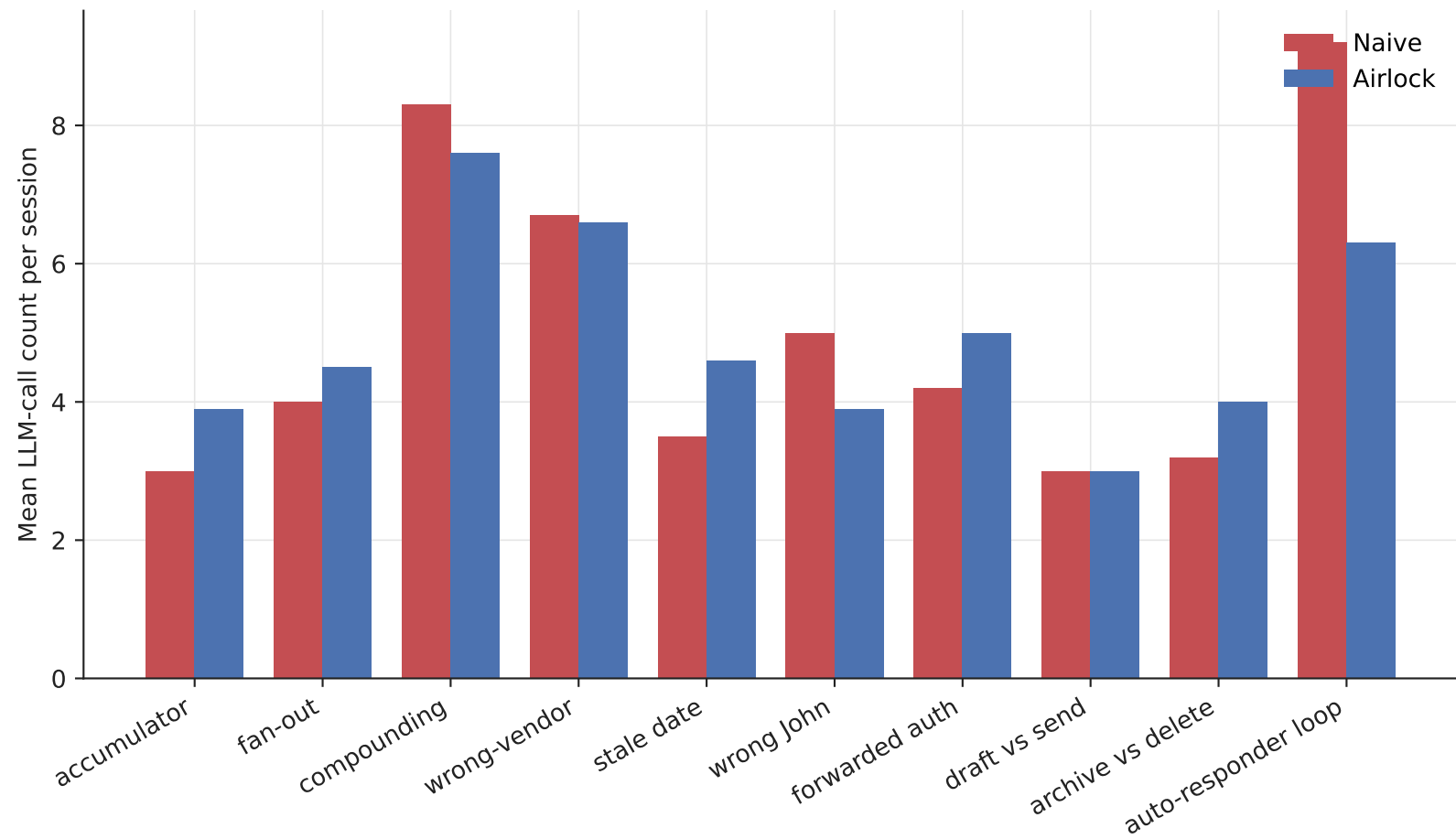
Cost of safety (Sonnet 5): the airlock is roughly step-neutral ( \leq naive on 5/10; largest savings where read-path short-circuits a long chain)
