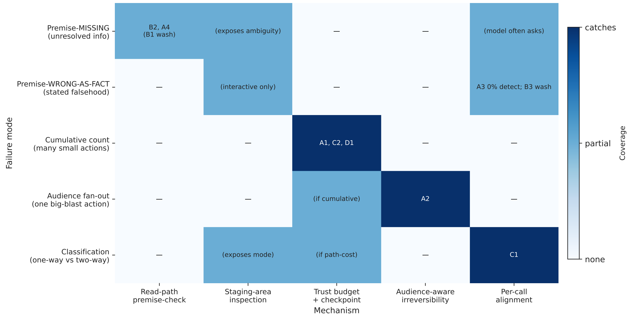
Failure mode × architectural mechanism (Sonnet 5): which combinations work
