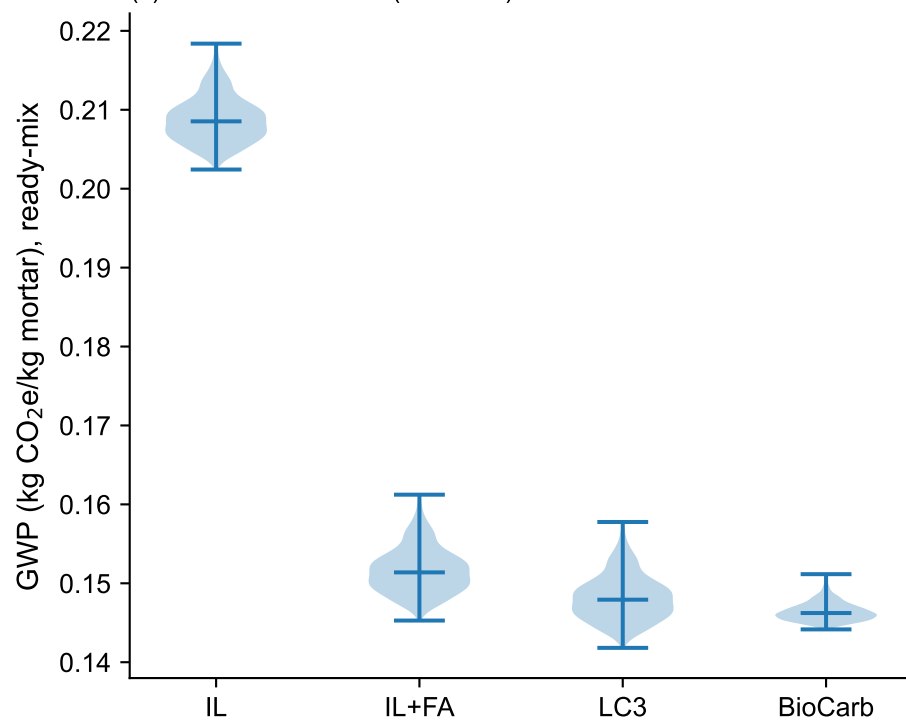
(c) Monte Carlo GWP (n = 1000)
