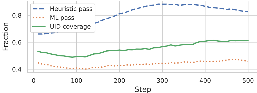
Figure 7: Acceptance rates of the ACR self-distillation pipeline over training for Llama-3.1-8B-Instruct: fraction of batches passing the heuristic filter, passing the machine-learning (ML) filter, and meeting unique identifier (UID) coverage.
