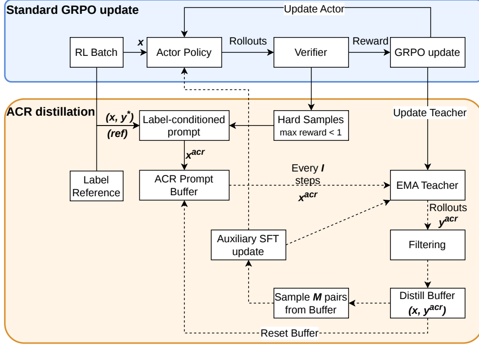
Figure 2: MinervaRL overview separating the standard GRPO loop from the auxiliary ACR path. Solid arrows show the synchronous training flow, while dashed arrows show the periodic ACR distillation pass.
