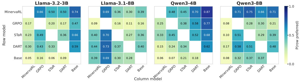
Figure 3: GPT-5.2 pairwise response-quality preferences for backbone-specific model groups. Each cell reports the probability that the row model is preferred over the column model, with ties retained in the denominator.
