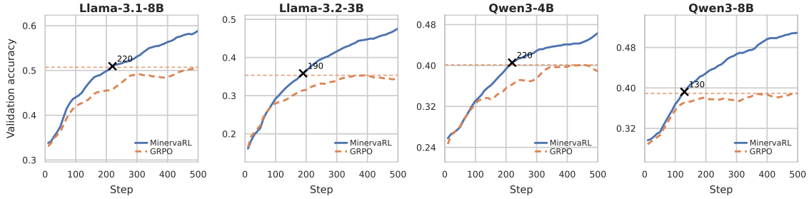
Figure 5: Validation accuracy over training. Curves are 5-step rolling means; dashed lines mark the best GRPO accuracy, and crosses mark the first MinervaRL step that reaches it.
