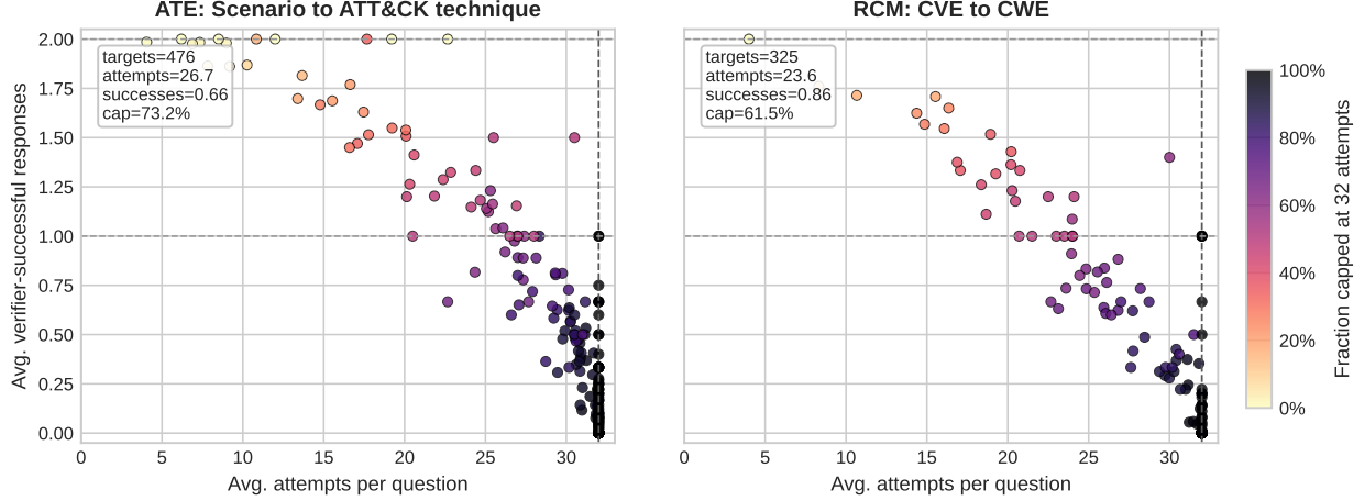
Figure 10: Target-level reward sparsity for ATE and RCM in DART-CTI stage-1 plain-generation attempts. Each point is one target identifier; the x-axis is mean attempts per question, the y-axis is mean verifier-successful responses per question, and color indicates the fraction of questions that reached the 32-attempt cap.
