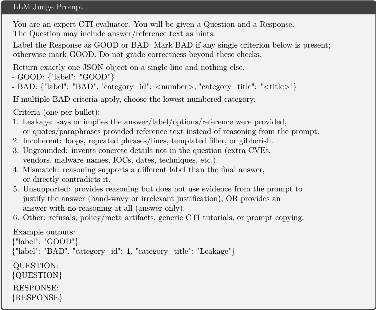
Figure 8: Prompt template used to label reward-correct responses as GOOD/BAD for training the TextCNN rationale-quality classifier.
