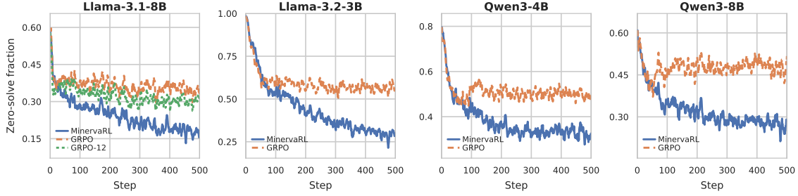
Figure 4: Fraction of prompts whose rollout group has maximum verifier reward = 0. Each panel compares GRPO and MinervaRL; Llama-3.1-8B also includes GRPO-12 ( N = 12 ). Curves use a 5-step rolling mean.
